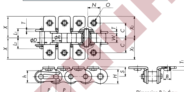
K1NM Attachment
