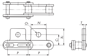
EP Attachment
