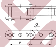
GNK1 Attachment
