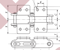
SK2 Attachment
