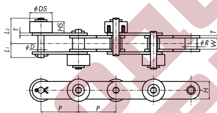
Chain with Brake
