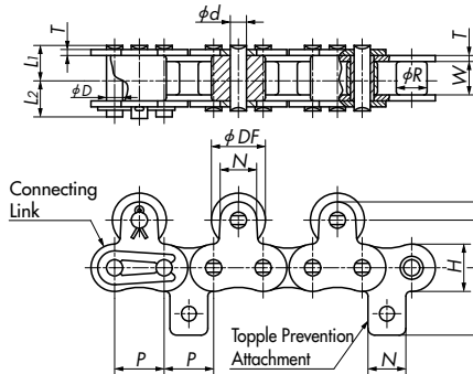
Installation of Top Rollers: Outer Link
