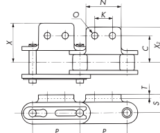
SA2 Attachment
