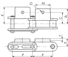
SA1 Attachment
