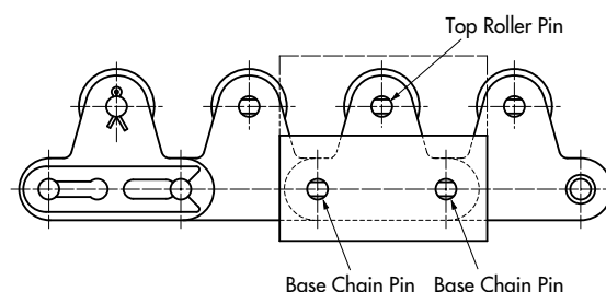
Figure 15: Removing Base Chain Pins
