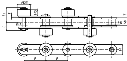
Base Chain R Roller Staggered Installation (Type I)
