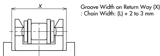
Figure 22: Return Way
