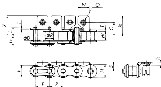
A1NM Attachment
