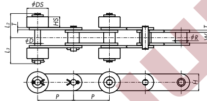
Crosswise Installation (Type II)
