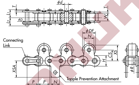
Installation of Top Rollers: Inner Link
