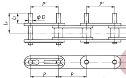
EP Attachment
