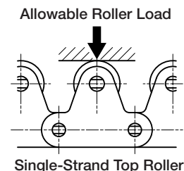
Single-Strand Top Roller
