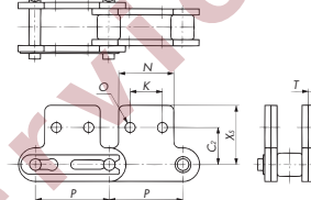
SK2 Attachment
