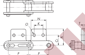
GNK1 Attachment
