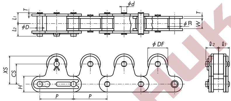
Base Chain S Roller
