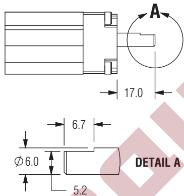
SHAFT ONLY.
