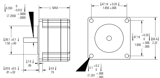
NEMA 23 (56mm)
