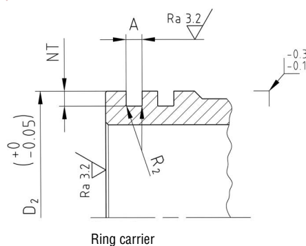
Ring carrier
