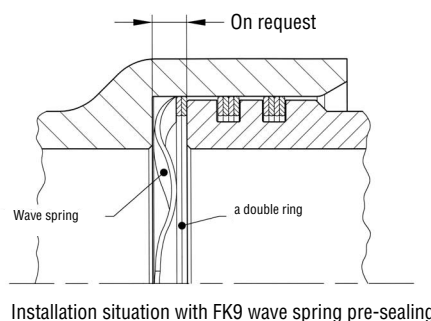
Installation situation with FK9 wave spring pre-sealing
